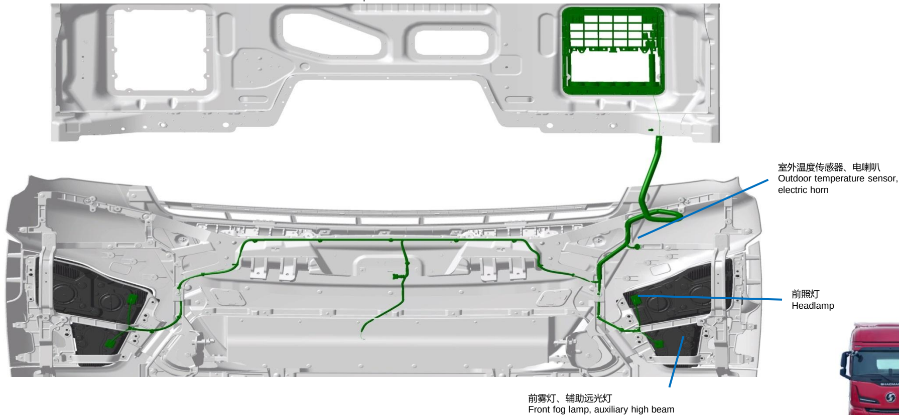
保险杠线束 Bumper harness
