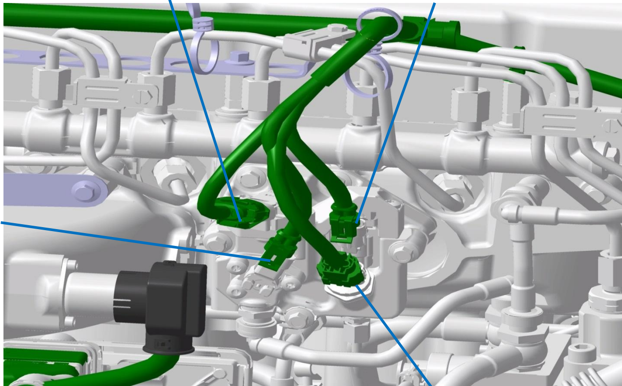
HCI下游温度传感器 HCI downstream temperature sensor
