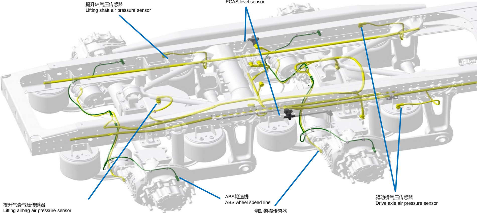
制动磨损传感器 Brake wear sensor
