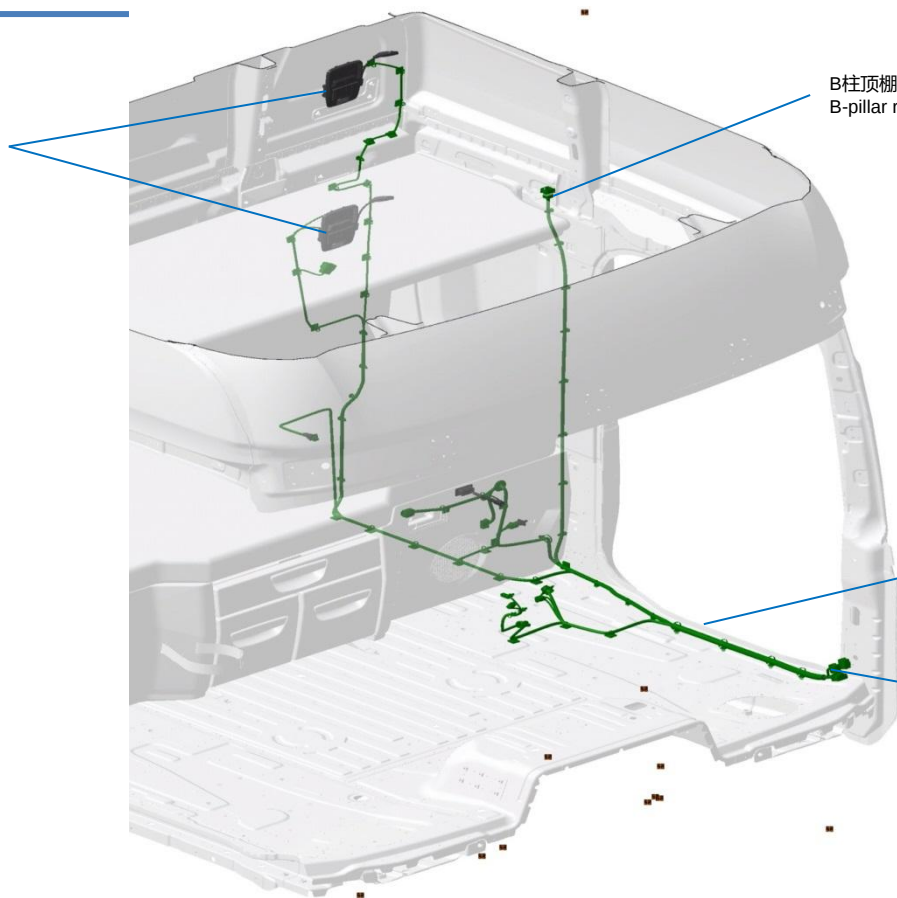
左地板线束 LH floor wire harness
