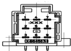
插接器X2 A插件 Connector X2 plug-in A
